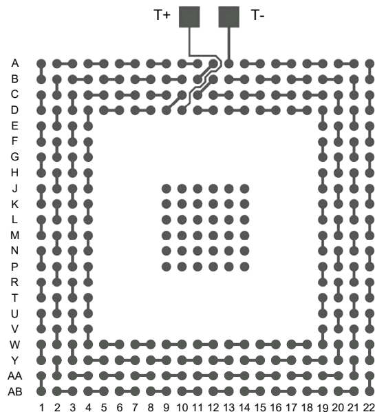
AFTER MOUNTING
